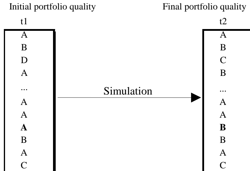
Figure A.3: Simulation Process
