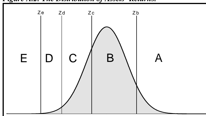
Figure A.2: The Distribution of Assets' Returns.
